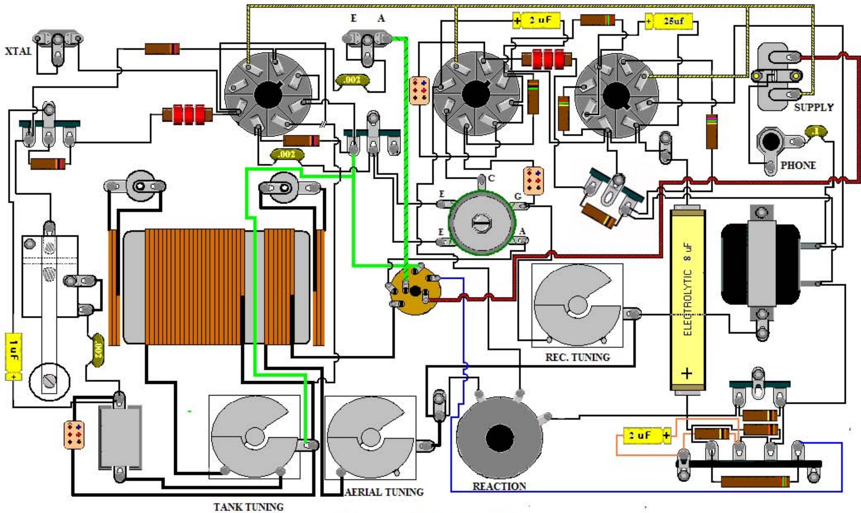
Paraset Wiring Diagram
